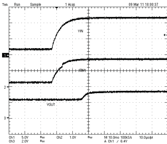
Figure 48. Prebias Startup With V_{IN}
