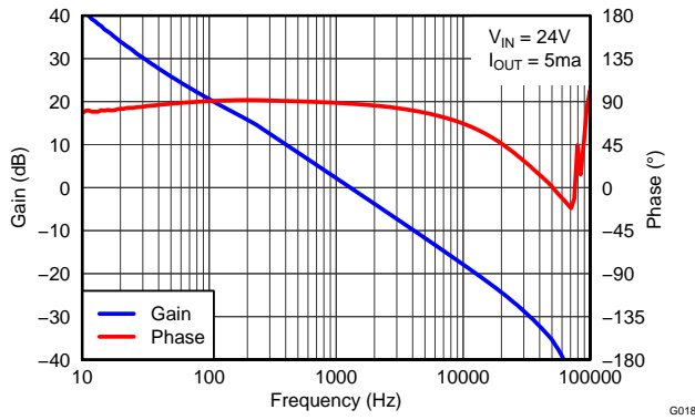
Figure 40. Gain vs Phase
