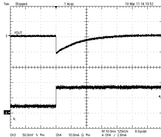
Figure 43. Load Transient
