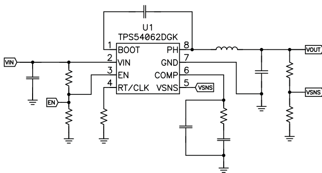
SIMPLIFIED SCHEMATIC
